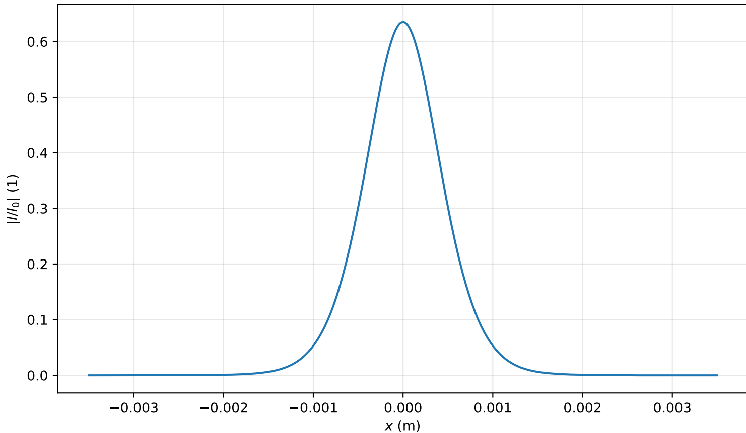
Intensity profile I(x, y = 0, z = 3.184m)/I_0 , P_{in}=0.6P_{cr} , artificial time
